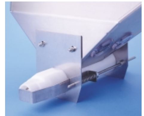
Pellet shutoff closeup
