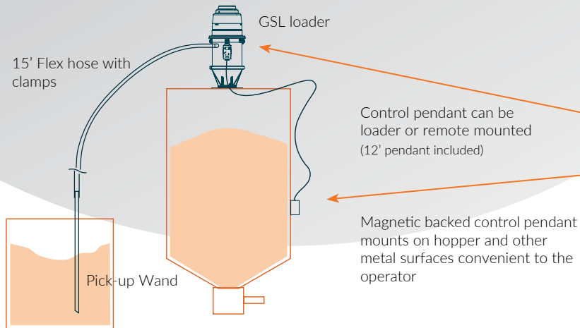
Full-featured control includes load time, no-load alarm, alarm light and silencer as well as proportioning and purging.
