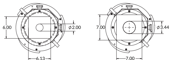
Mounting Patterns
